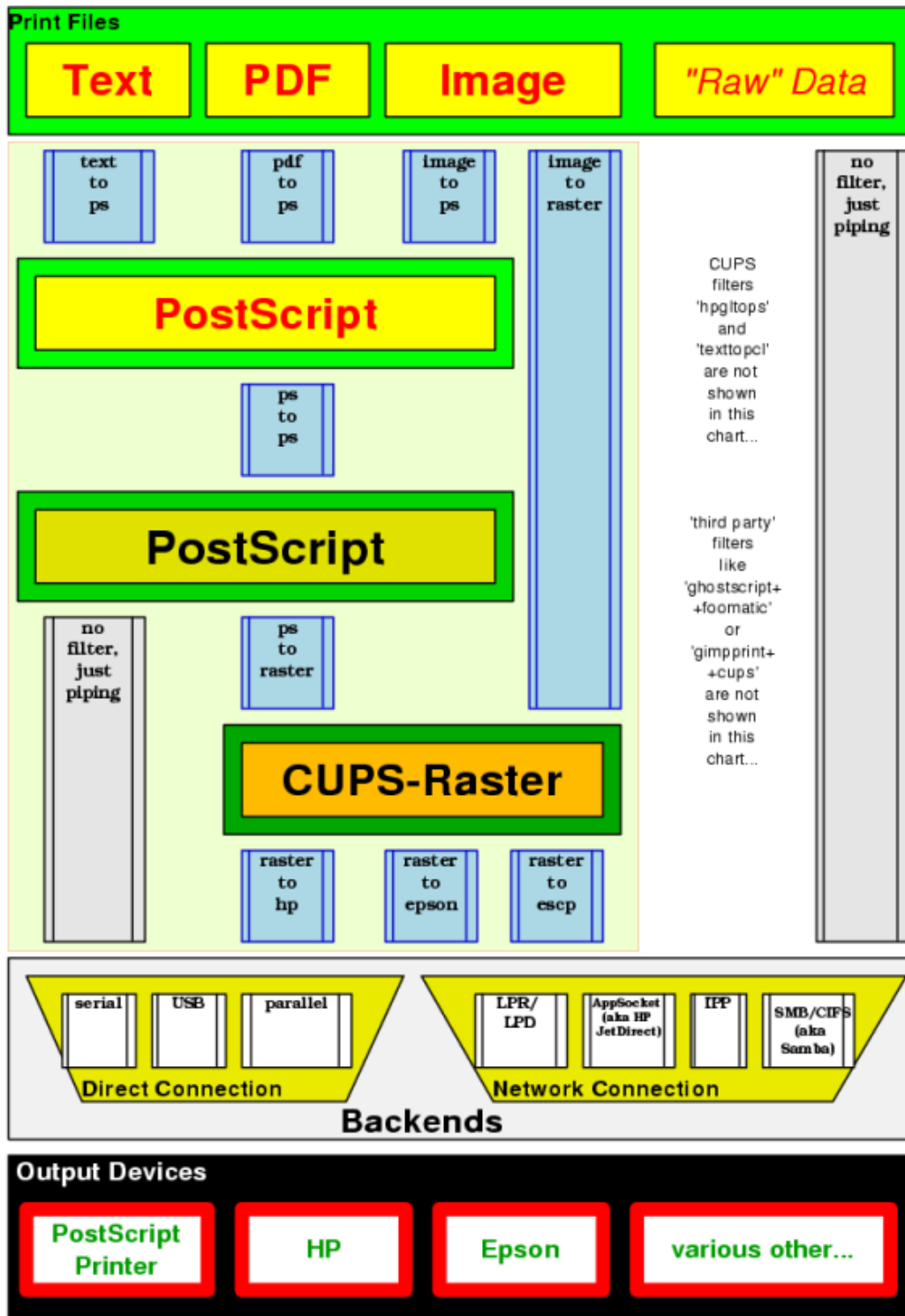
CUPS: "Core" Filter and Backend Architecture
