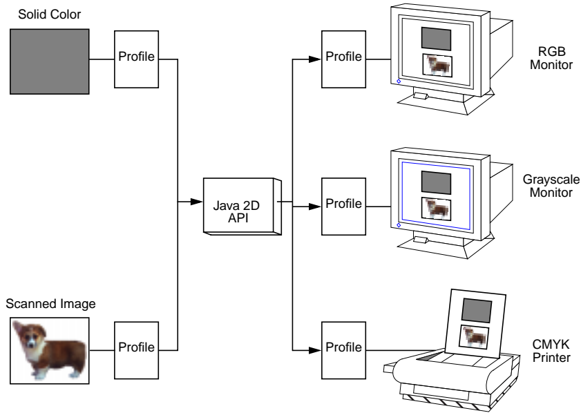
Figure 6-3 Using Profiles to Map Between Color Spaces
