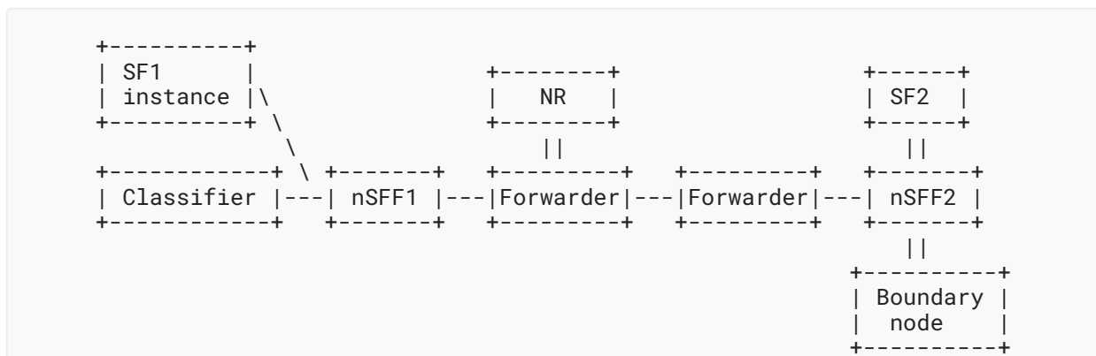
Figure 3: High-Level Architecture
